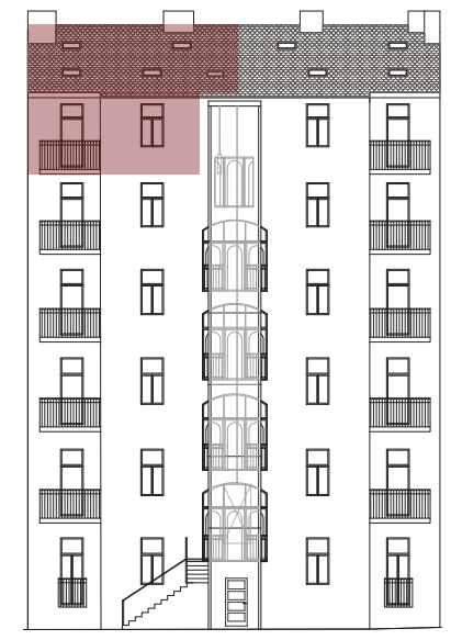
BACK-WESTERN ELEVATION
