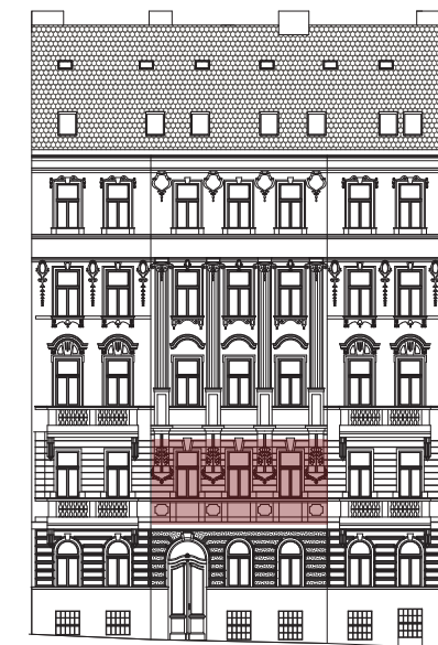
FRONT-EASTERN ELEVATION
